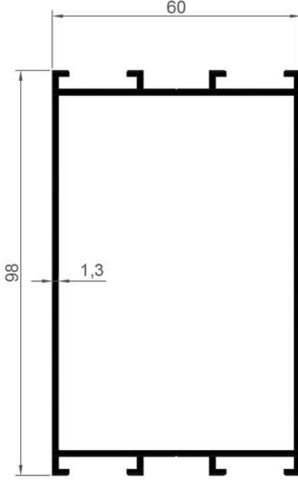
16378 1,225 Kg/Mt
