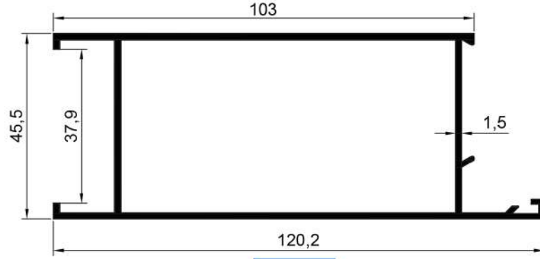
16608 1,315 Kg/Mt
