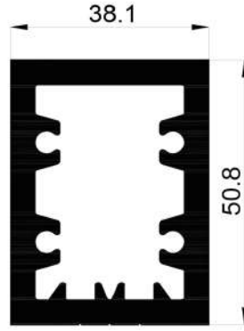
16717 2,436 Kg/Mt
