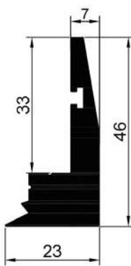
16324 1,108 Kg/Mt
