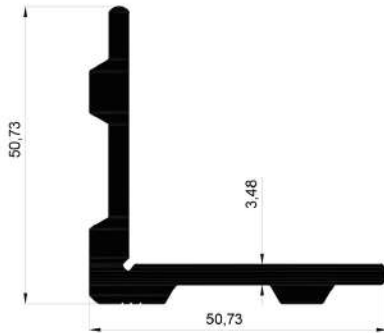
16723 1,226 Kg/Mt
