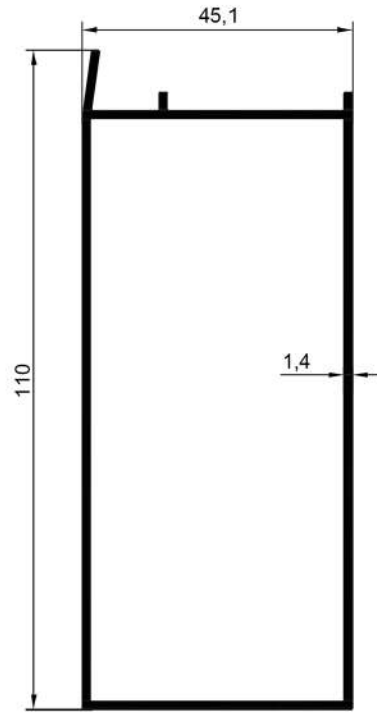
16313 1,100 Kg/Mt
