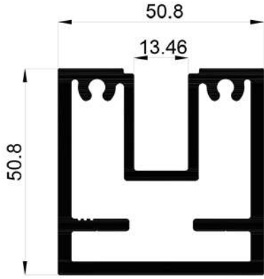
16711 2,262 Kg/Mt
