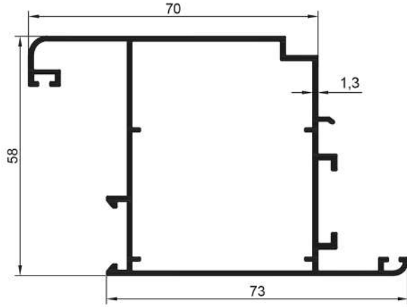
16434 1,050 Kg/Mt
