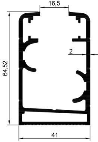
16851 1,410 Kg/Mt
