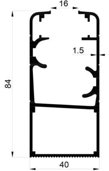
16338 1,477 Kg/Mt
