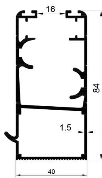
16337 1,551 Kg/Mt
