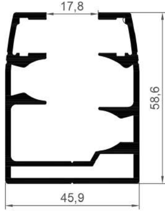
16280 1,471 Kg/Mt
