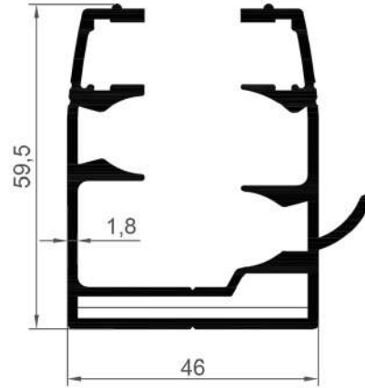
16278 1,550 Kg/Mt
