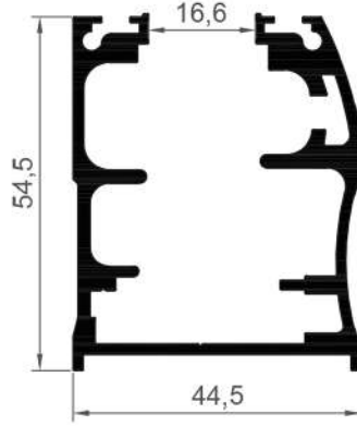
16301 1,340 Kg/Mt
