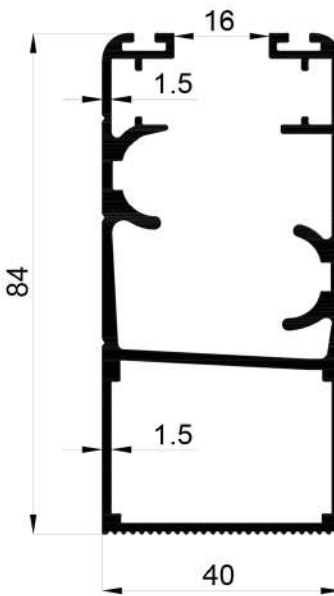
16336 1,506 Kg/Mt
