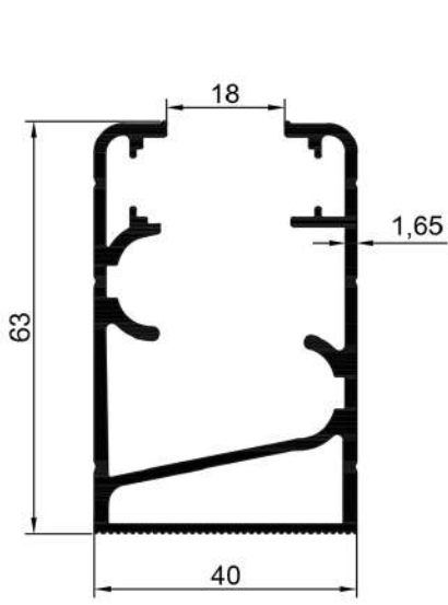
16447 1,220 Kg/Mt
