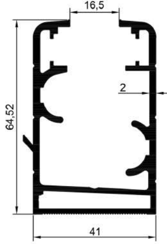
16852 1,430 Kg/Mt
