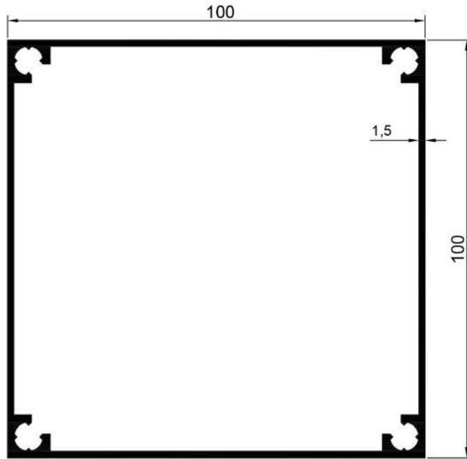
16705 1,868 Kg/Mt
