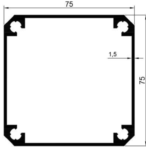
16704 1,628 Kg/Mt
