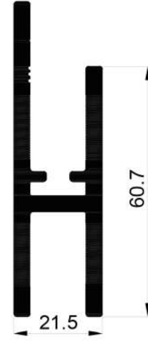
16712 1,671 Kg/Mt
