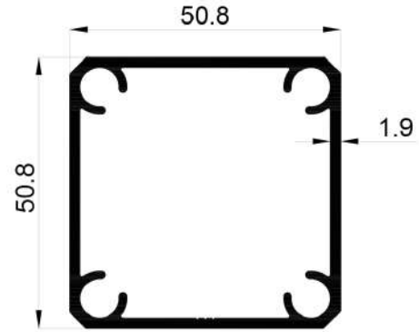
16730 1,154 Kg/Mt
