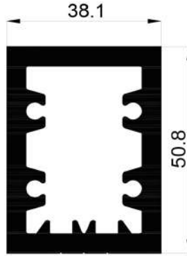
16717 2,436 Kg/Mt
