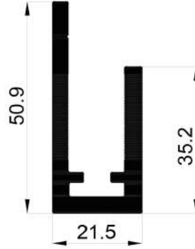
16709 1,109 Kg/Mt
