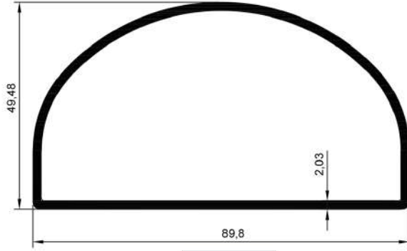
16713 1,304 Kg/Mt
