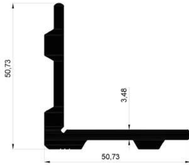
16723 1,226 Kg/Mt
