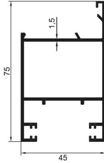
16505 1,085 Kg/Mt
